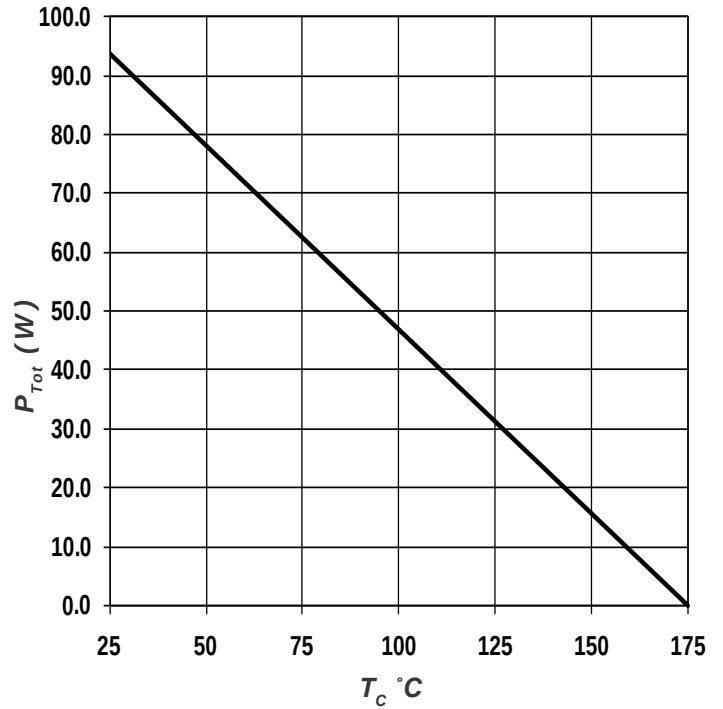
Figure 4. Power Derating
