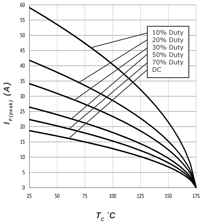
Figure 3. Current Derating
