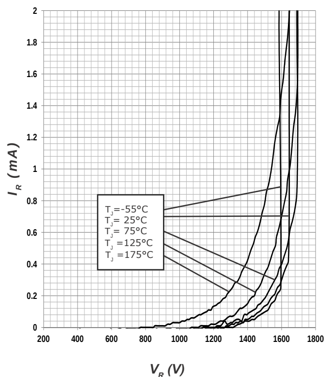
Figure 2. Reverse Characteristics
