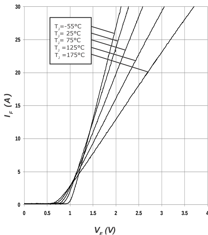
Figure 1. Forward Characteristics
