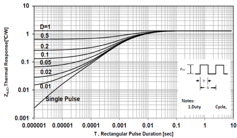
Fig 8: Transient Thermal Impandance
