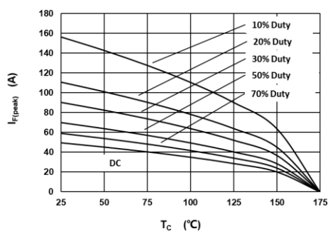
Fig 3: Current Derating
