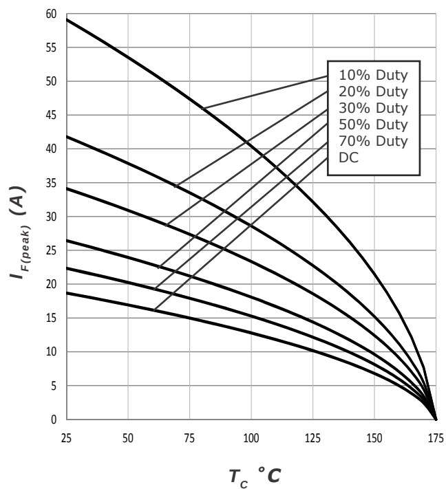
Figure 3. Current Derating
