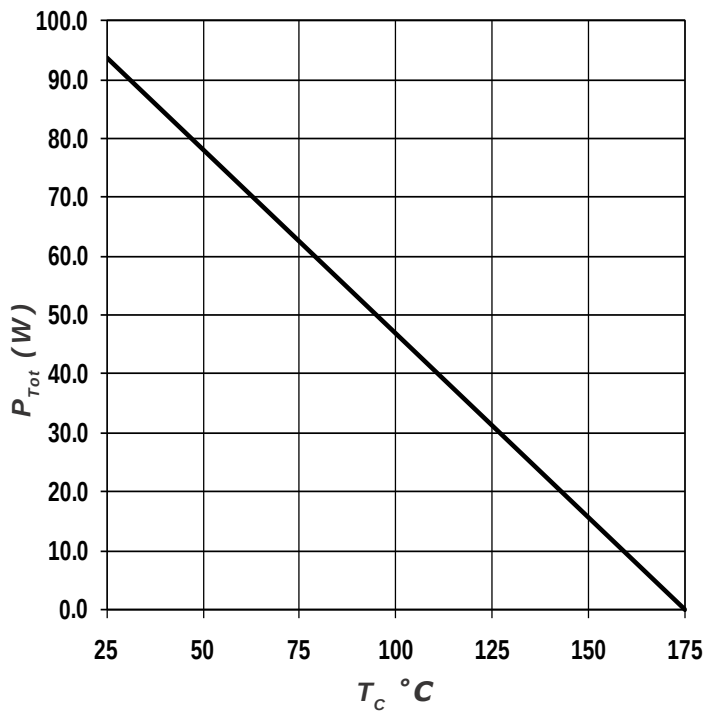
Figure 4. Power Derating
