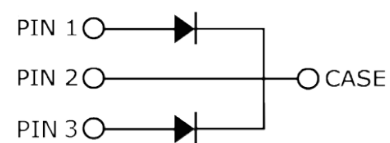
TO-247
