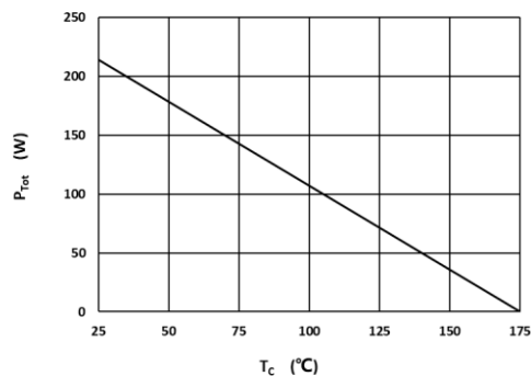
Fig 4: Power Derating
