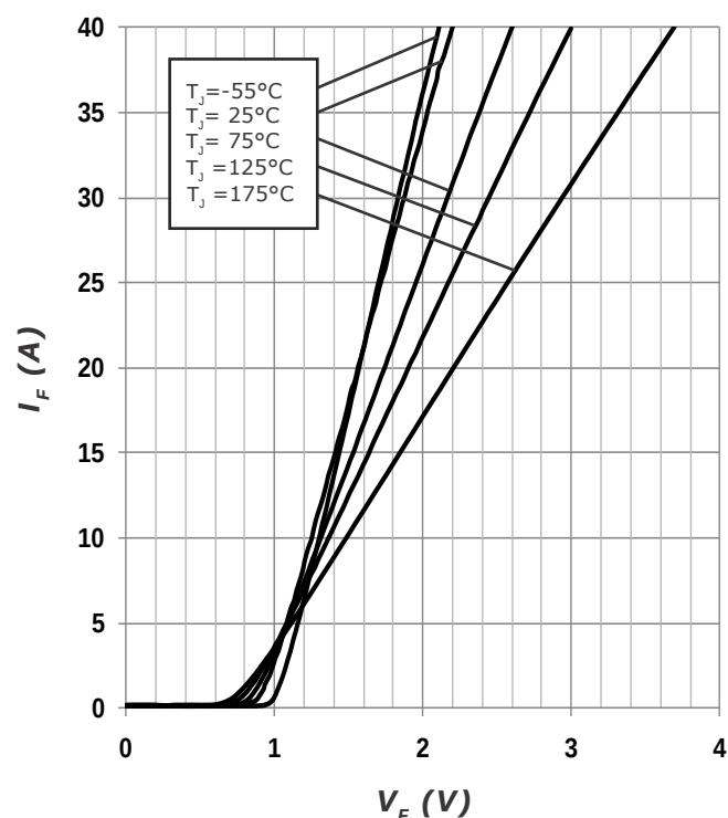
Figure 1. Forward Characteristics
