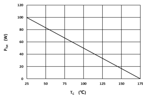
Fig 4: Power Derating
