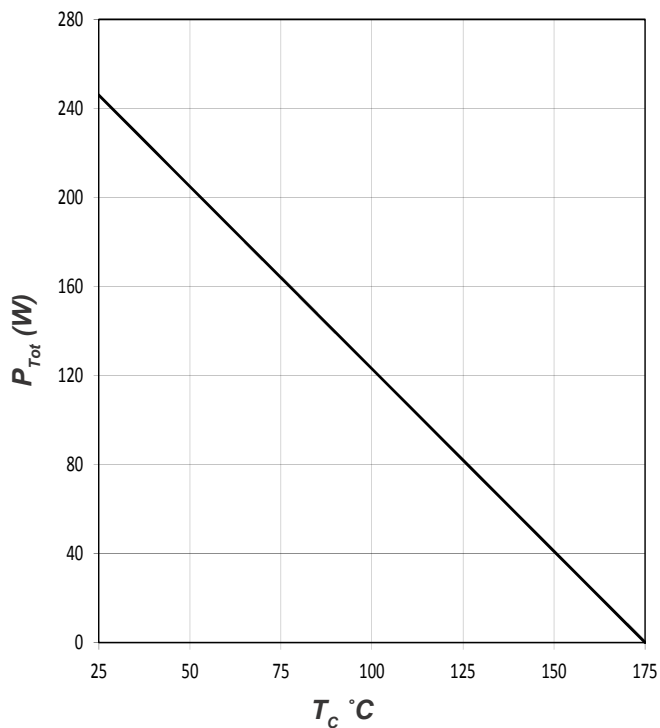
Figure 4. Power Derating
