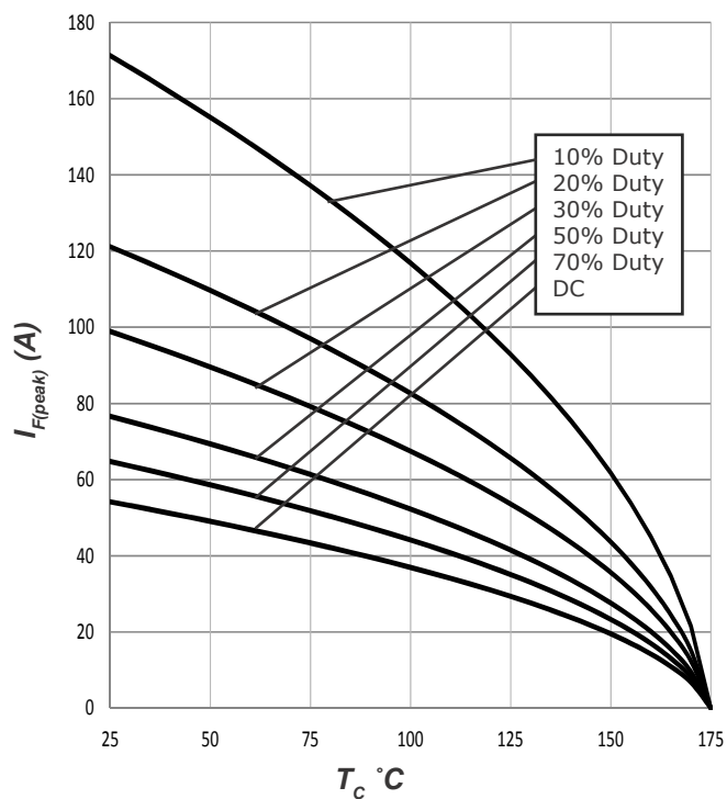
Figure 3. Current Derating
