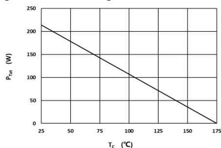
Fig 4: Power Derating
