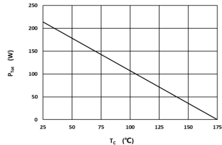
Fig 4: Power Derating
