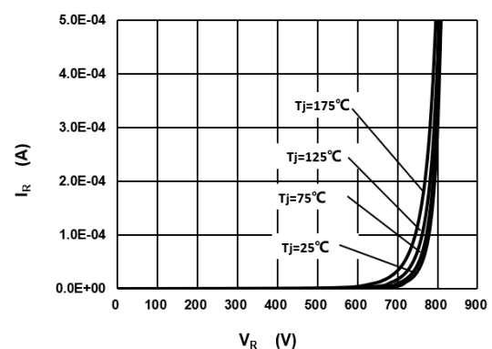
Fig 2: Reverse Characteristics
