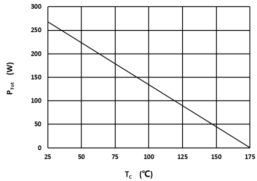
Fig 4: Power Derating
