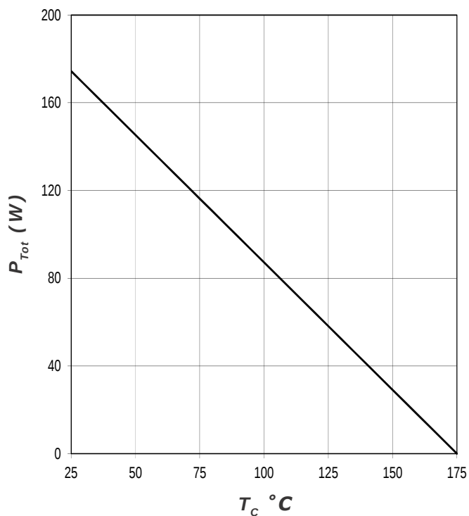
Figure 4. Power Derating
