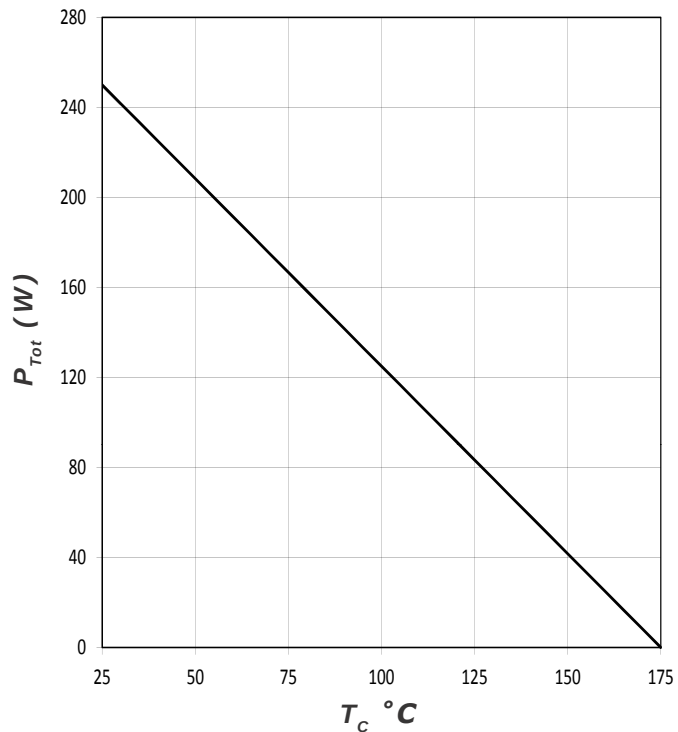
Figure 4. Power Derating
