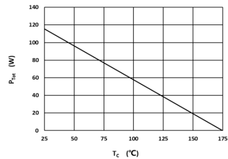
Fig 4: Power Derating
