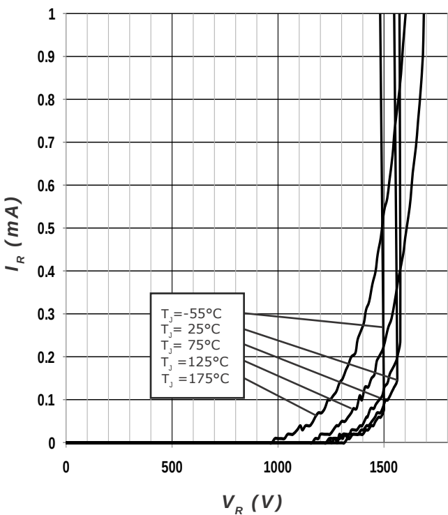
Figure 2. Reverse Characteristics
