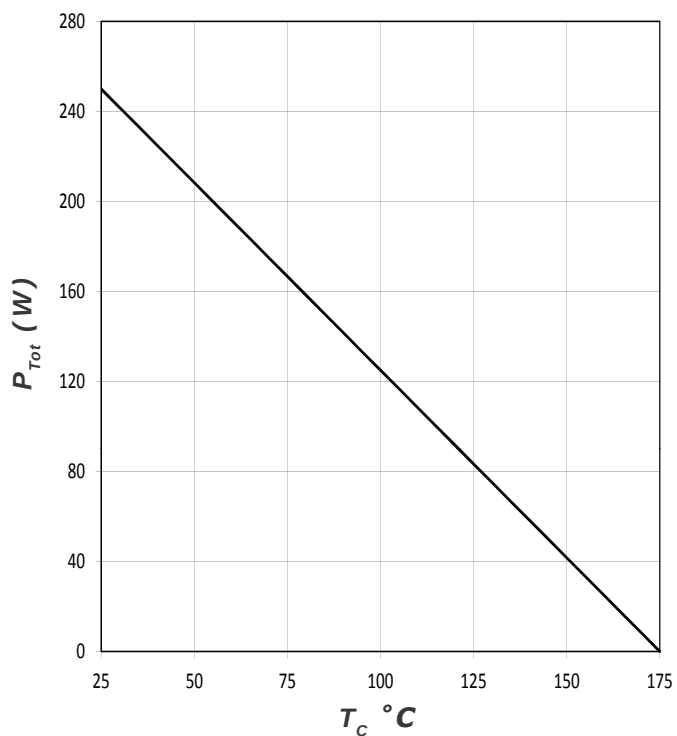
Figure 4. Power Derating
