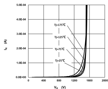
Fig 2: Reverse Characteristics
