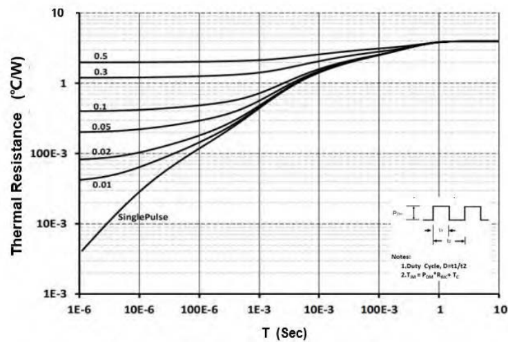
Fig 8: Transient Thermal Impedance
