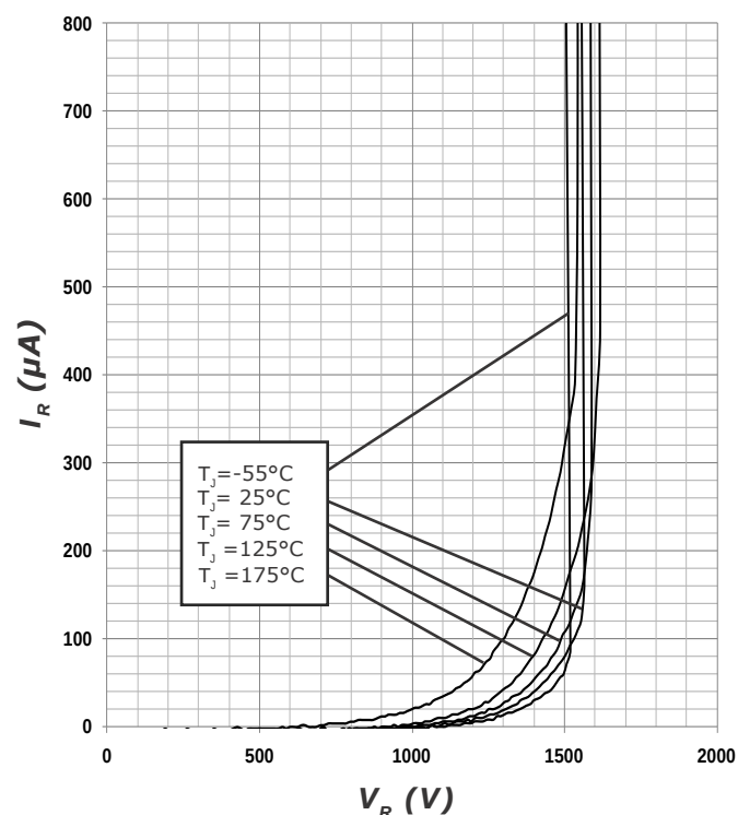
Figure 2. Reverse Characteristics
