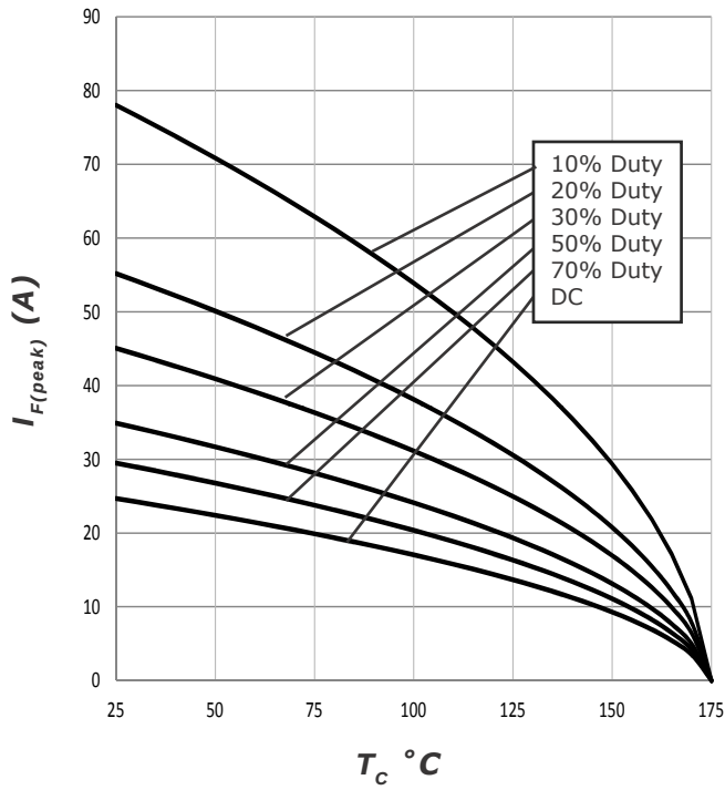
Figure 3. Current Derating
