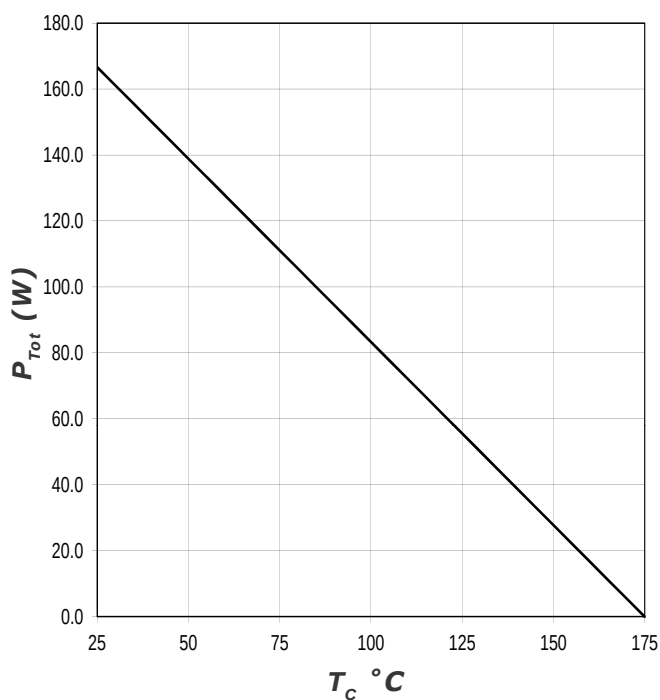
Figure 4. Power Derating
