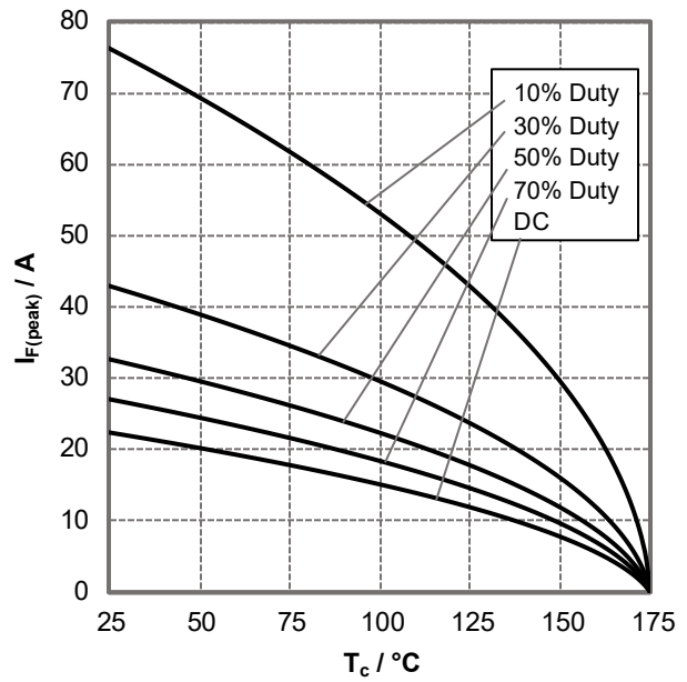
Figure 4. Current Derating
