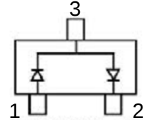
BAT54SW
