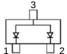
BAT54AW
