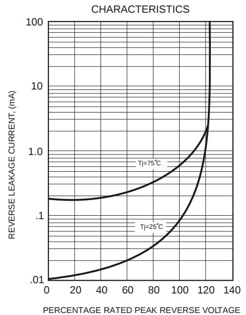
FIG.5 - TYPICAL REVERSE
