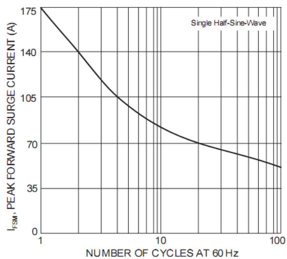
Fig. 8 Max Non-Repetitive Peak Forward Surge Current
