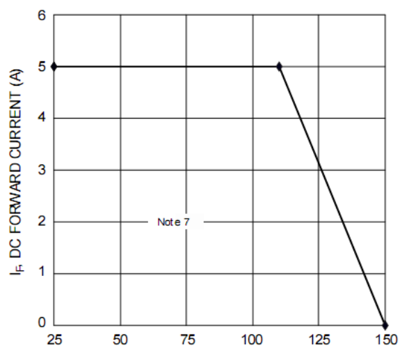
Figure 7 DC Forward Current Derating
