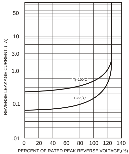
FIG.3-Typical Reverse Characteristics
