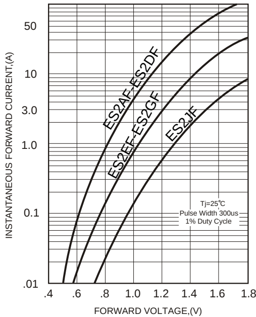
FIG.2-Typical Forward Characteristics
